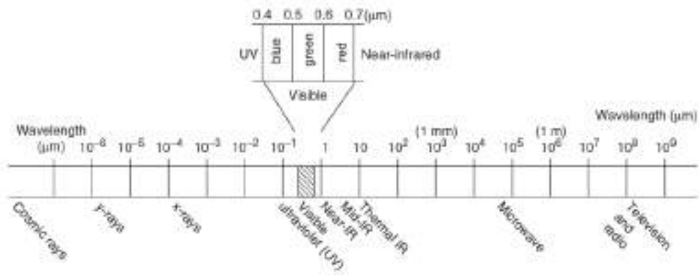
Figure 2.3: Electromagnetic spectrum components
